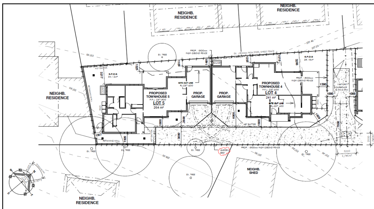
Figure 3: Site plan 2
