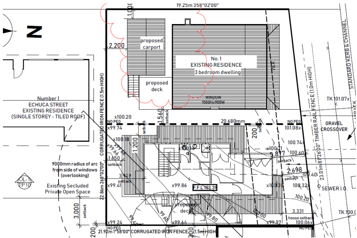
Figure 7: First floor / site layout plan
