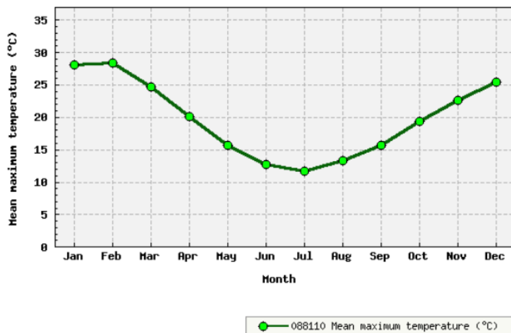
Figure 3 - Average daily maximum temperatures recorded at Castlemaine Prison (BOM, 2016)
