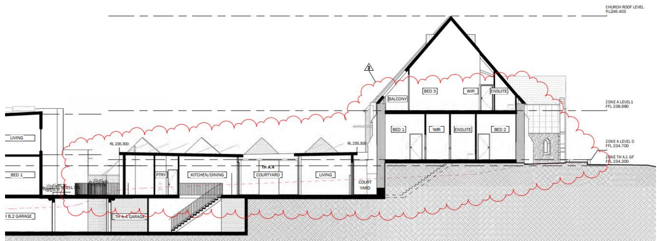
Figure 15: Section plan showing connection of new extension to existing church
