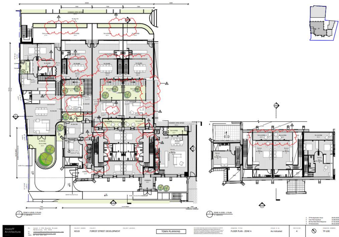
Figure 6: Proposed ground and first floor plans of original church and additions
