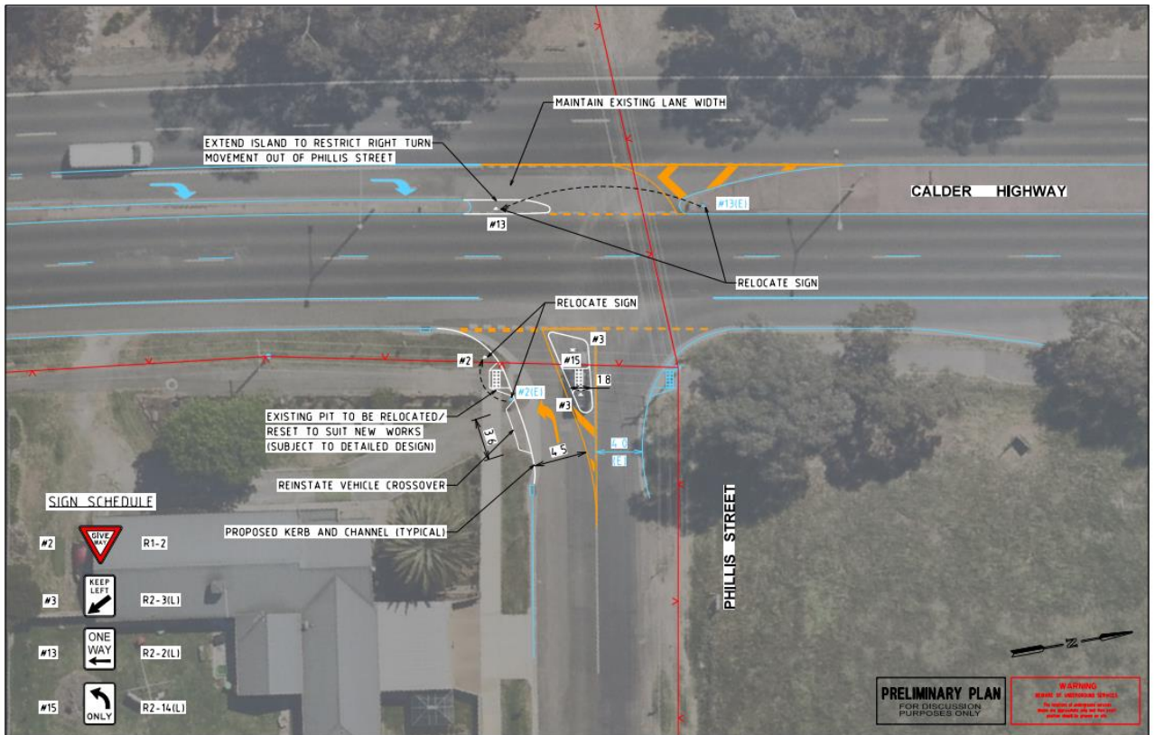
Figure 14. Concept layout plan for Phillis Street/Calder Highway intersection
