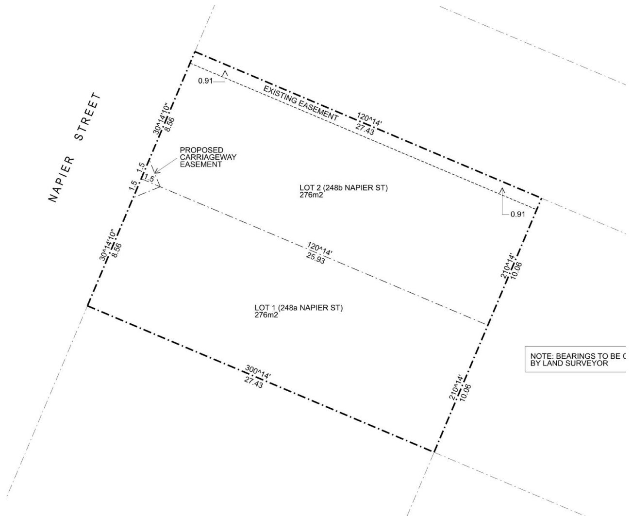
Figure 8: Proposed subdivision
