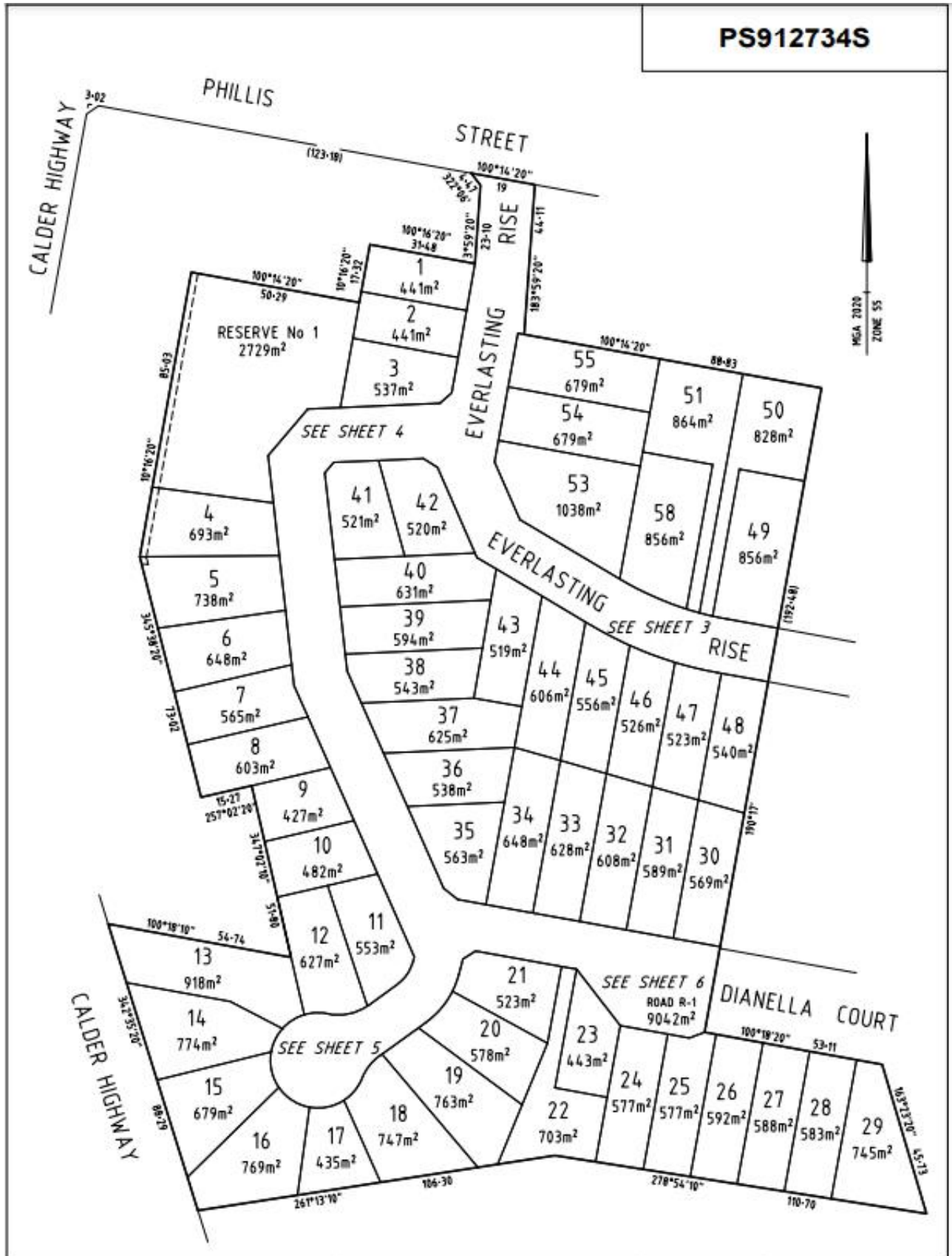
Figure 9. Proposed plan of subdivision
