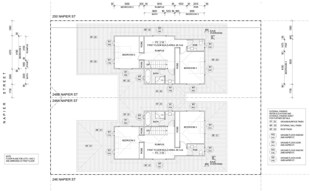
Figure 6: Proposed second storey plan
