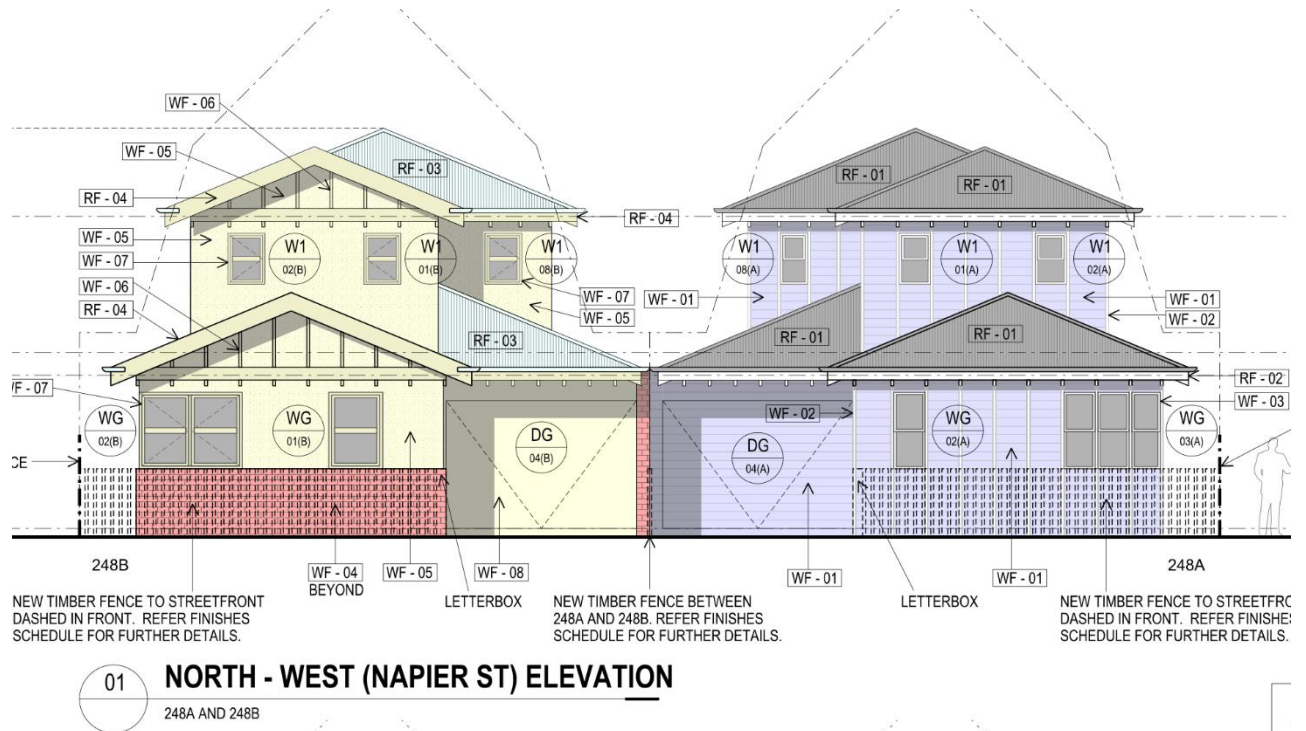
Figure 7: Front elevation
