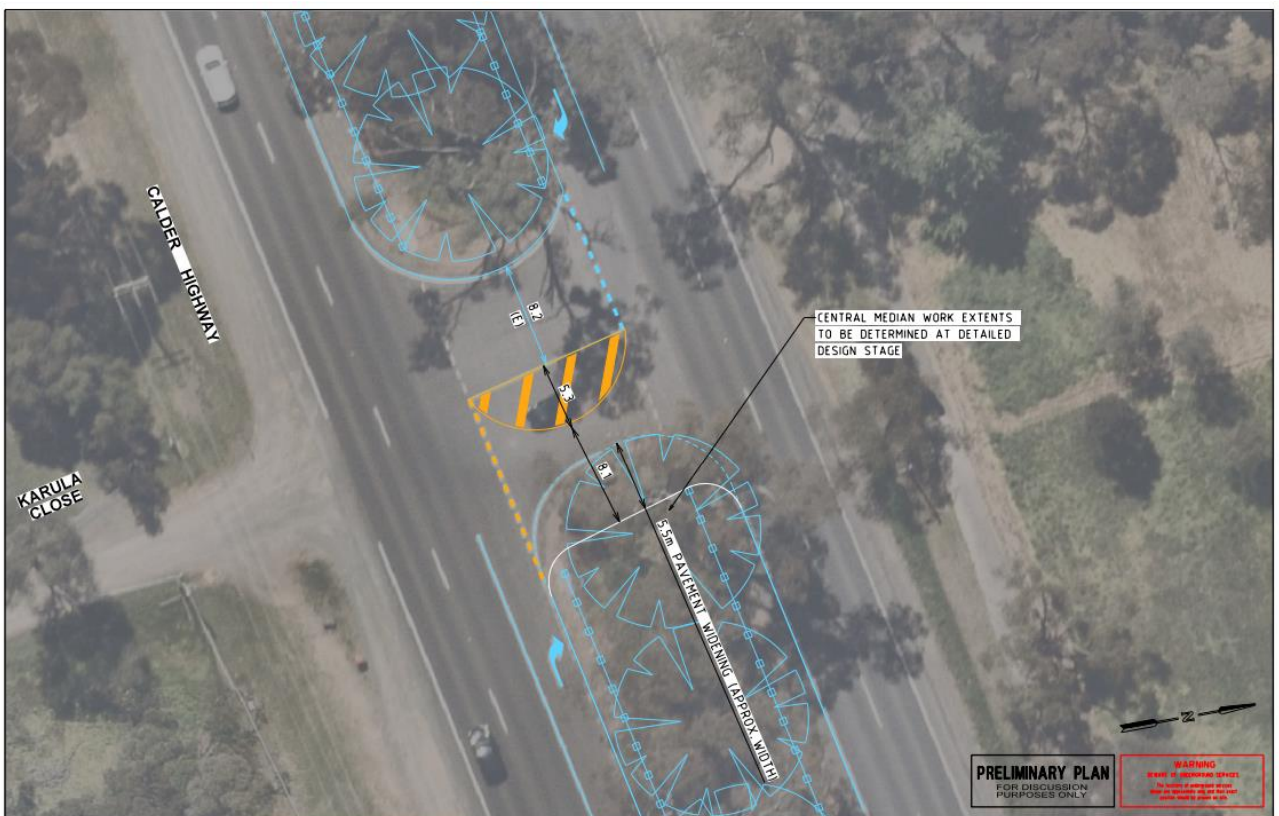
Figure 15. Concept layout plan for Karula Close/Calder Highway intersection
