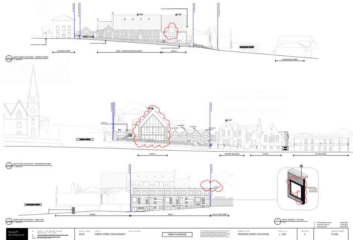
Figure 11: Forest Street, MacKenzie Street and View Lane elevations
