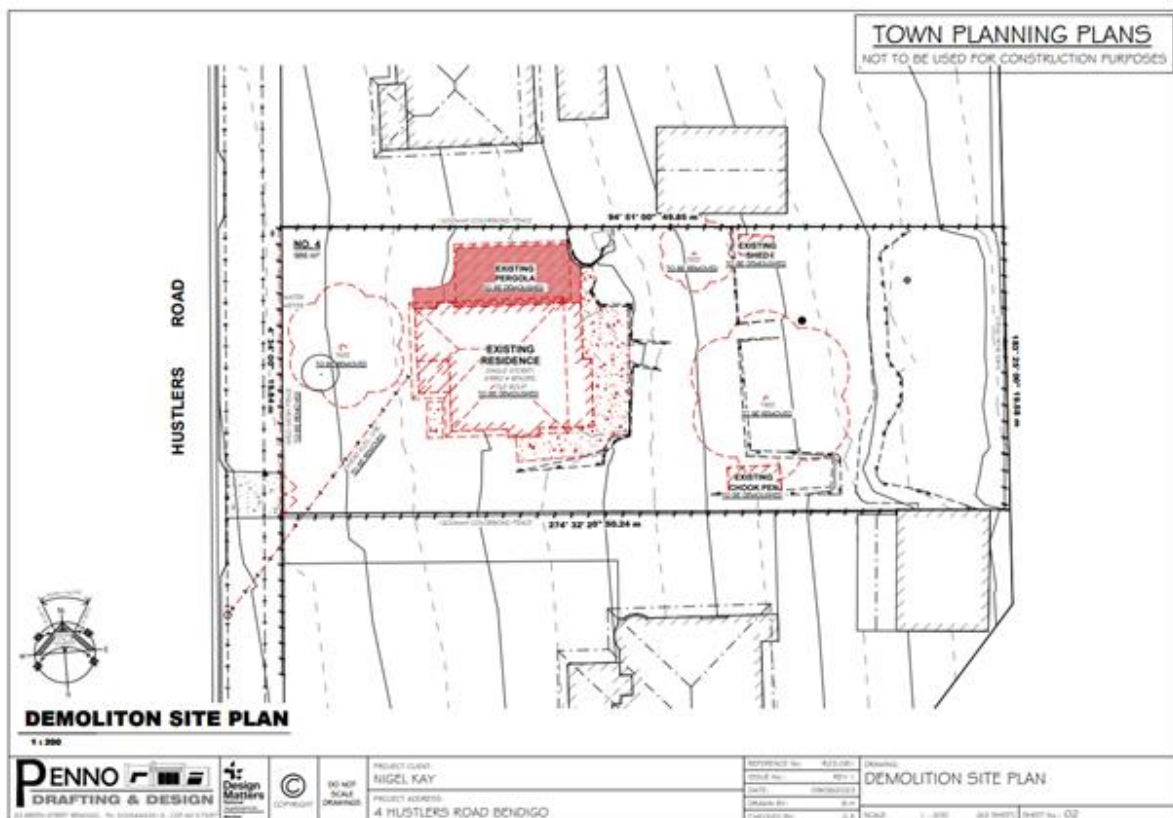
Figure 4: Existing conditions and proposed demolition plan
