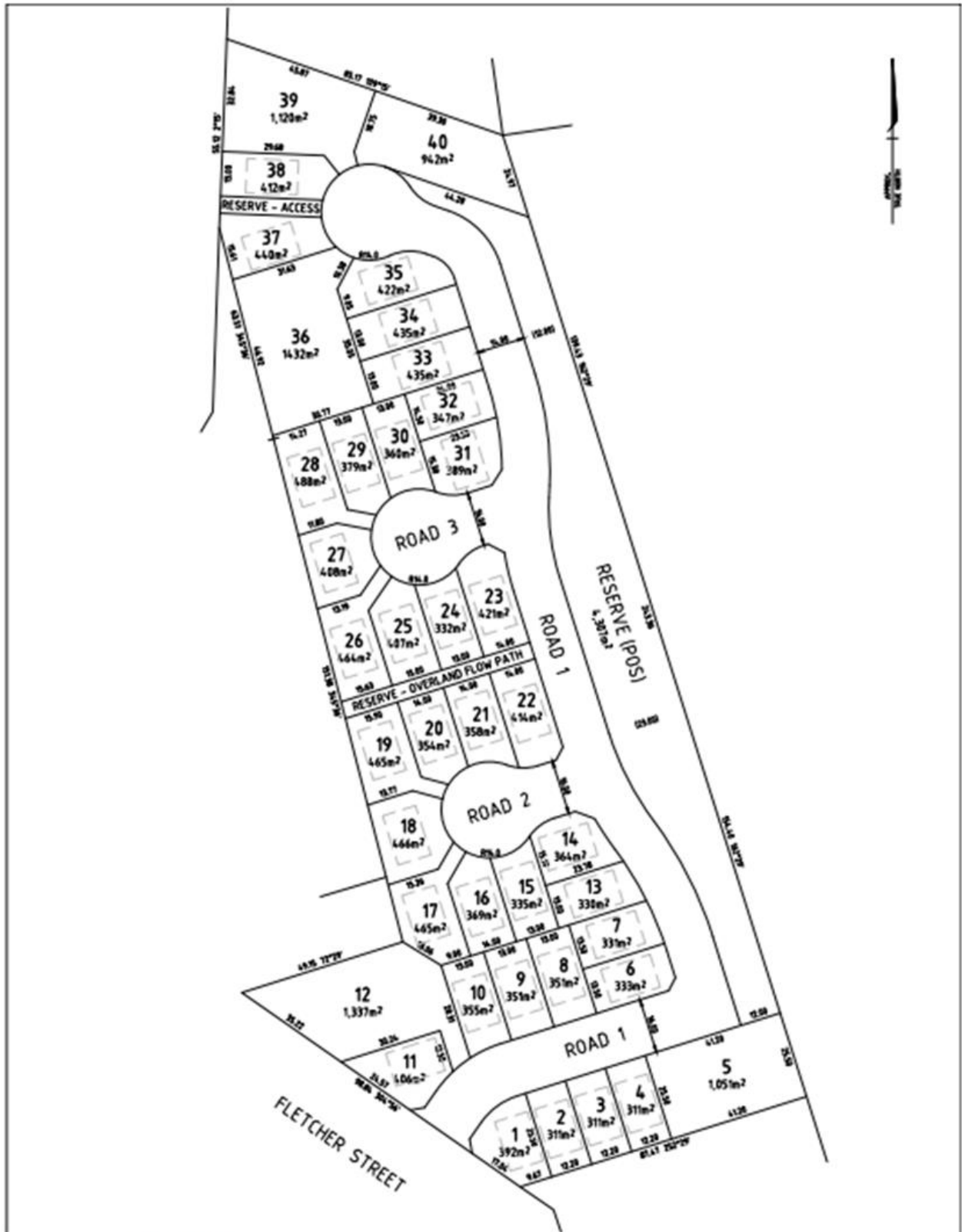
Figure 3: Proposed plan of subdivision.
