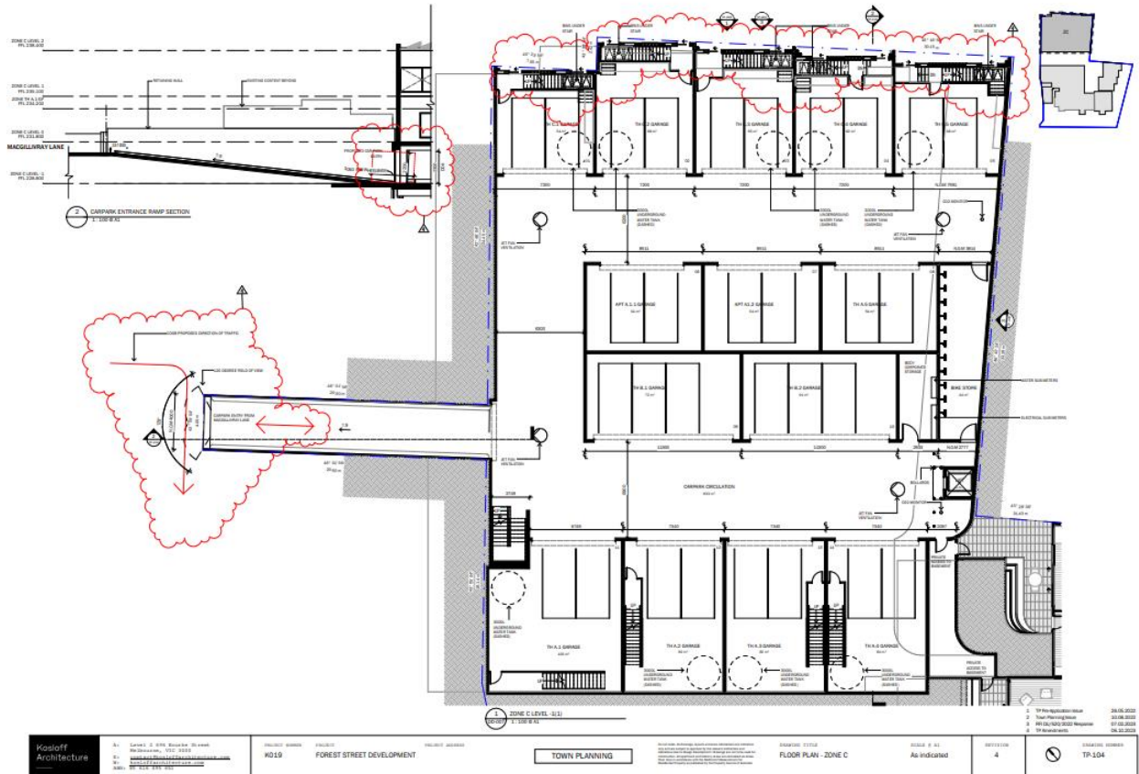
Figure 9: Proposed basement level
