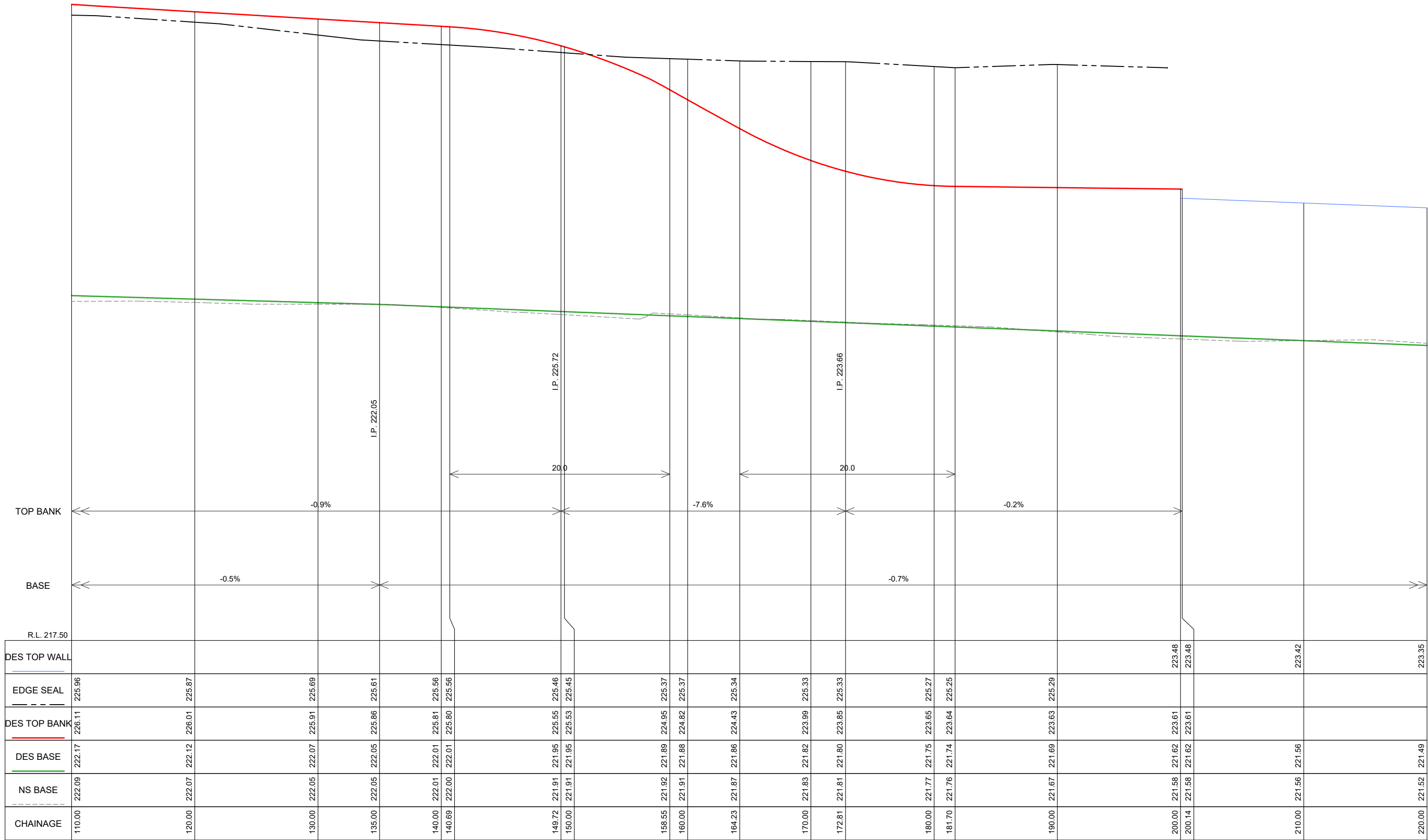
CREEK WALL LONGITUDINAL SECTION CH 110.000 To 220.000 SCALES: H 1:300 V 1:50 (A3)
