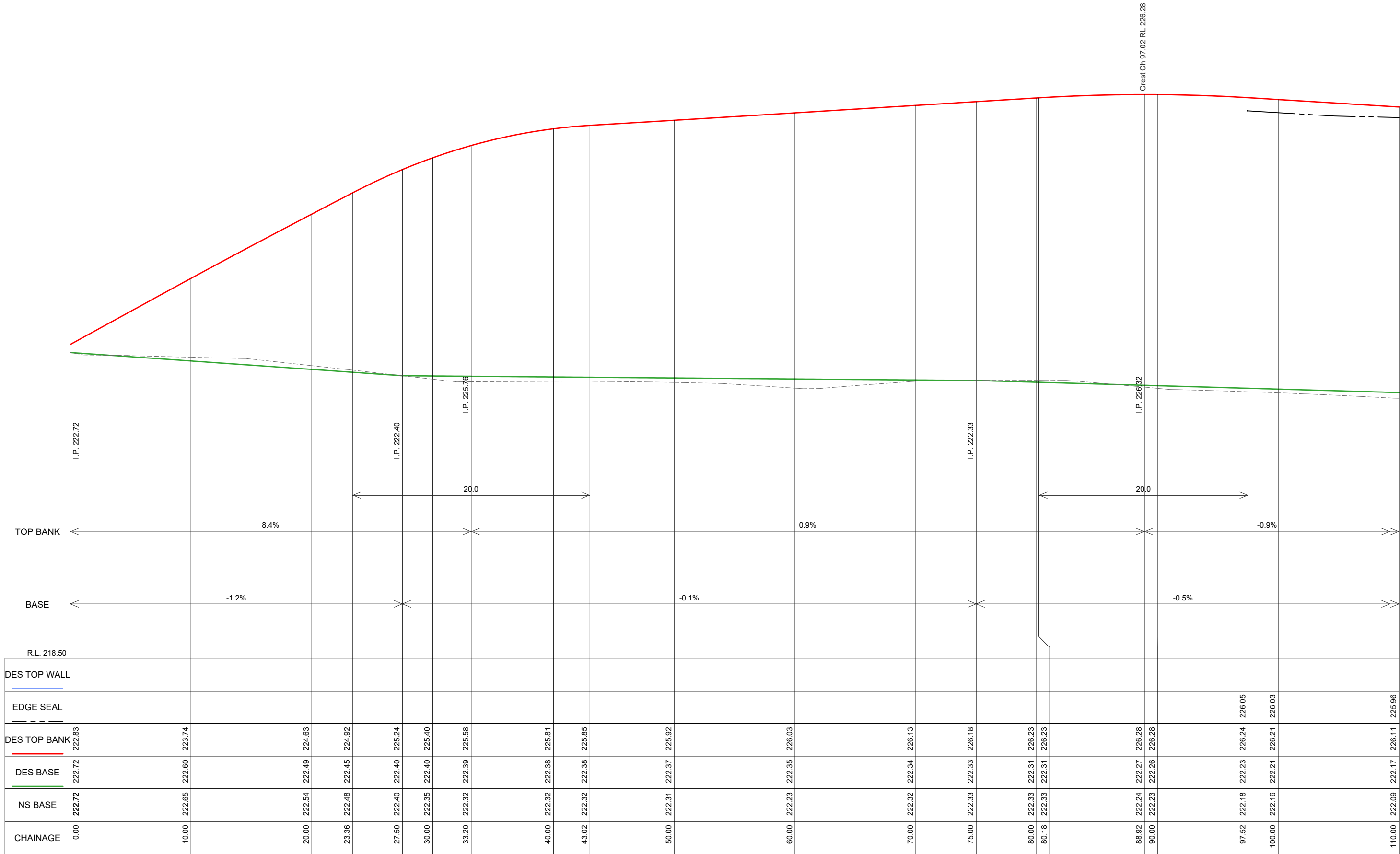
CREEK WALL LONGITUDINAL SECTION CH 0.000 To 110.000 SCALES: H 1:300 V 1:50 (A3)
