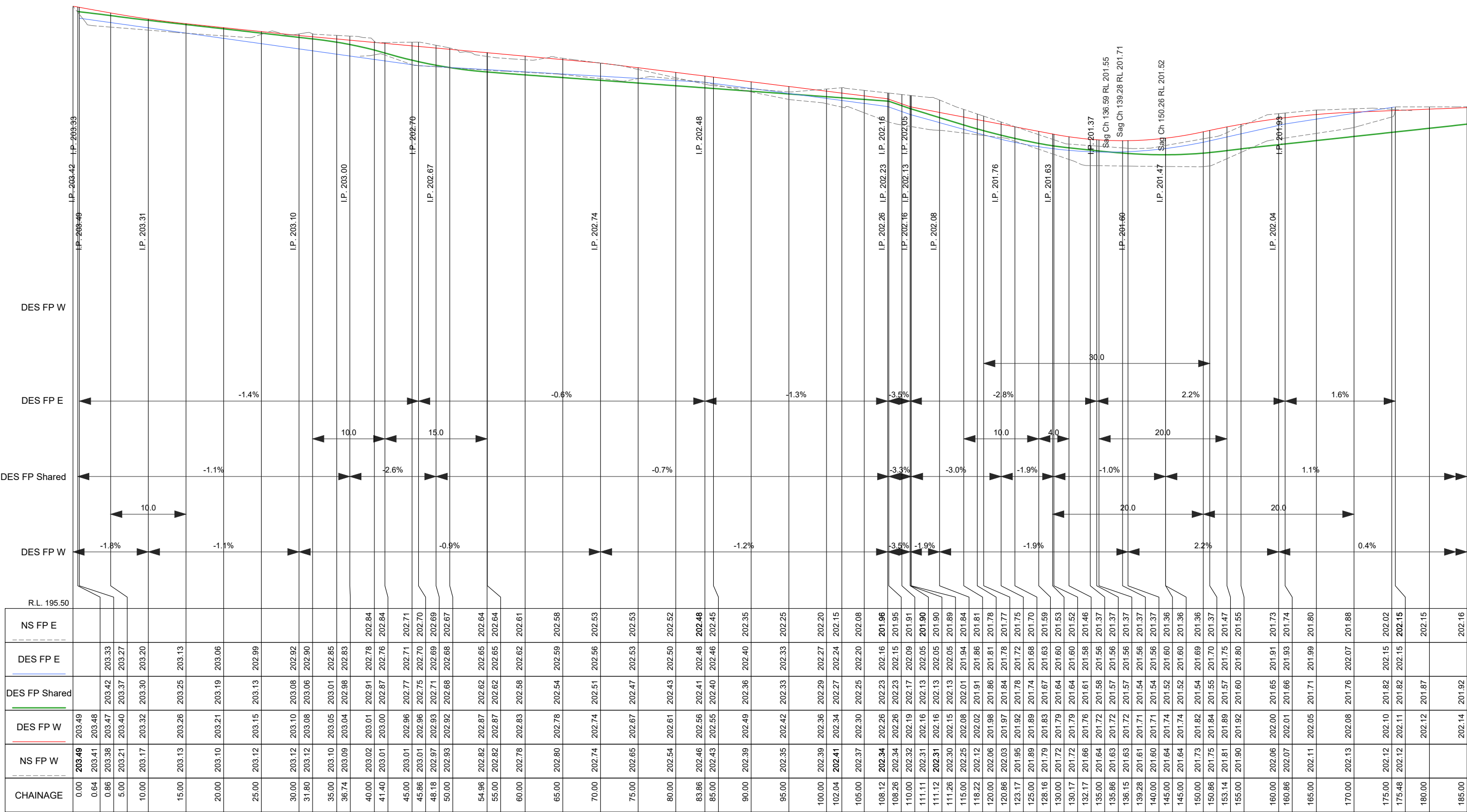
WELLESLEY LONGITUDINAL SECTION CH 0.000 To 185.000 SCALES: H 1:500 V 1:50 (A3)
