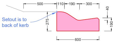
SM2 KERB PROFILE - IDM SD100 1:25
